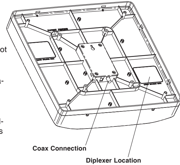
Figure 3 Antenna and Mount Assembled
