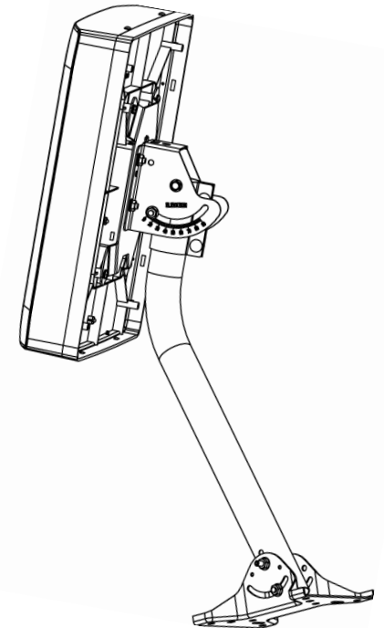
Figure 3 Antenna and Mount Assembled
